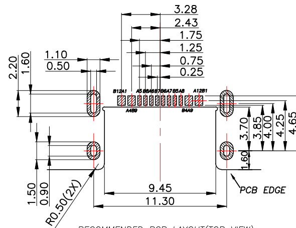
RECOMMENDED PCB LAYOUT(TOP VIEW) THICKNESS 1.0±0.10MM; DEFAULT TOLERANCE: ±0.05
